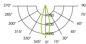
2x30° (1/10)
