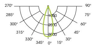
2x40° (1/10)
